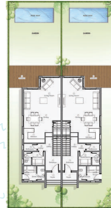
TWIN HOUSE GROUND FLOOR
